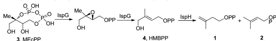
SCHEME 1. Formation of Isopentenyl Diphosphate ( 1 ) and Dimethylallyl Diphosphate ( 2 ) in the Nonmevalonate Pathway
