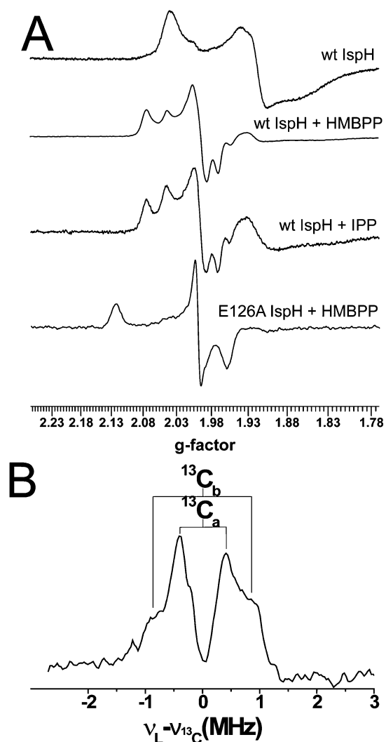
FIGURE 2. EPR and ENDOR results for IspH: (A) EPR spectra of IspH (and an E126A mutant) with and without ligands; (B) ENDOR spectrum with [u- ^{13}\text{C} ]- 26 . From ref 17 with permission. Copyright 2010 National Academy of Sciences.
