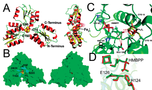
FIGURE 1. Structural results for IspH (LytB): (A,B) crystal structure results for Aquifex aeolicus IspH; (C) initial docking pose for HMBPP to oxidized IspH \text{Fe}_4\text{S}_4 cluster obtained by using the “open-form” structure; (D) Comparison of HMBPP bound to IspH from X-ray 16 (green) and docking 13 (red). From refs 13 and 16, with permission. Copyright 2008 American Chemical Society and 2010 National Academy of Sciences, U.S.A.
