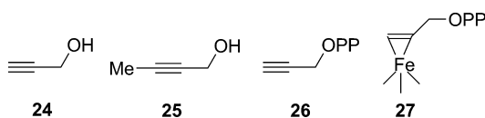
SCHEME 5. Acetylene Inhibitors of IspH and Proposed Binding Mode
