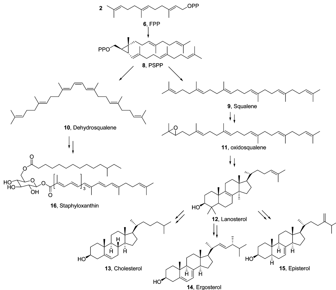
SCHEME 3. Formation of Triterpenes from Farnesyl Diphosphate (6)
